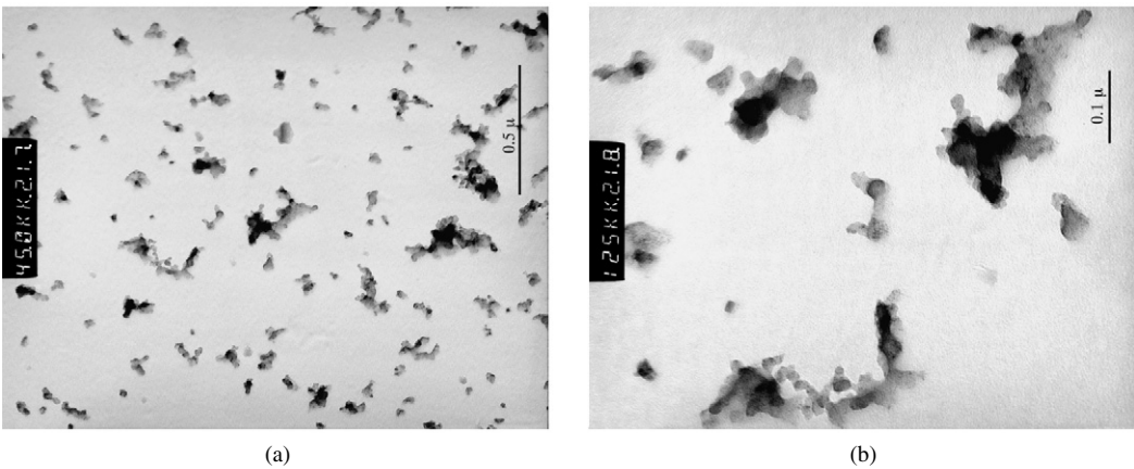
Fig. 14. (a) LPI stage 8 sample, 60 ppm doping, 6 kW load. (b) Zoom of same showing small metal agglomerates and very fine iron nanoparticles decorating a carbon agglomerate (upper right corner).
