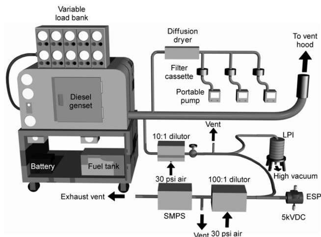
Fig. 1. Experimental setup.
