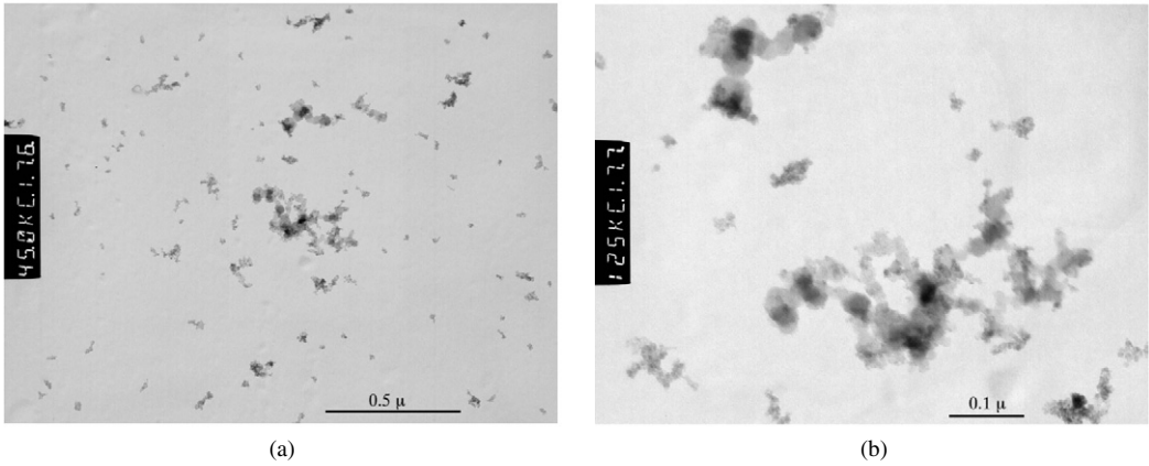
Fig. 13. (a) LPI stage 8 sample, 200 ppm doping, 6 kW load. (b) Zoom of same showing small iron agglomerates and iron nanoparticles decorating a carbon agglomerate.
