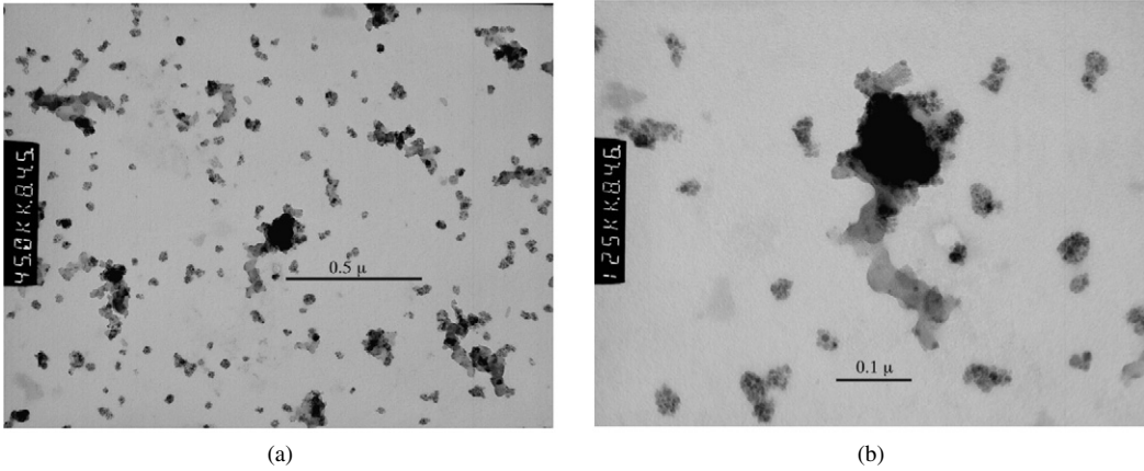
Fig. 12. (a) LPI stage 8 sample, 600-ppm doping rate, 0 kW engine load, showing prevalence of iron agglomerates (type 3) and combination iron/carbon particles. (b) Zoom of same shows primary iron nanoparticles (type 2) decorating a carbon agglomerate.
