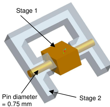
Fig. 1 In-mold assembled revolute joint.
