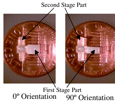
Fig. 6 In-mold assembled mesoscale revolute half joint
