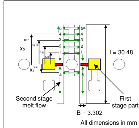
Fig. 5 Modular second stage mold design
