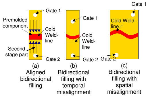
Fig. 3 Spatial and temporal gate misalignment
