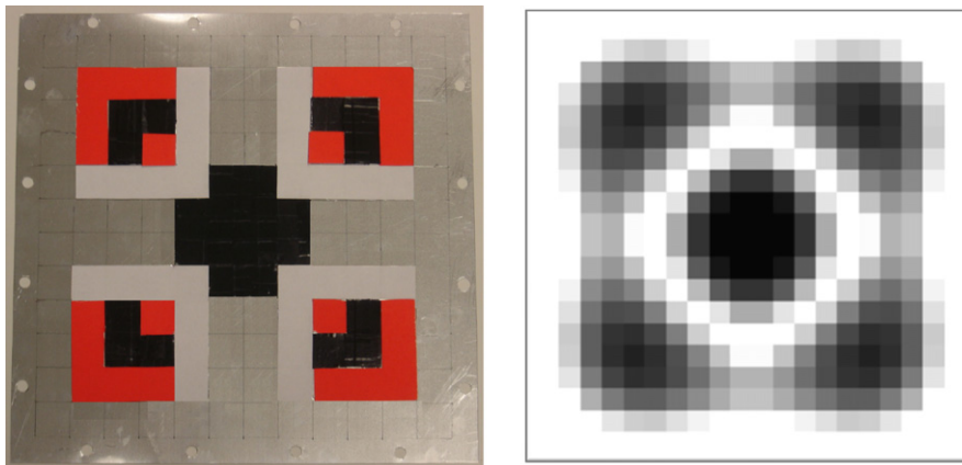
Fig. 13. Manufactured plate approximating the optimization results when targeting the first odd mode.
