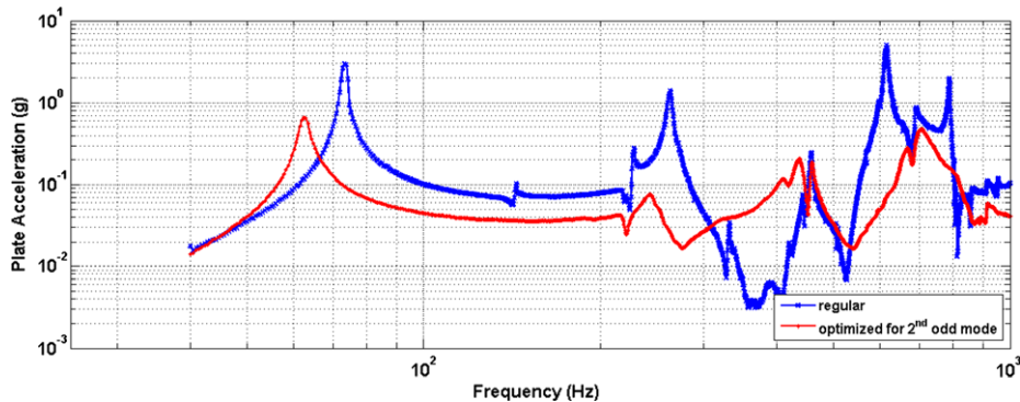
Fig. 19. Experimental accelerations of plain plate and topology optimized plate targeting second odd mode.
